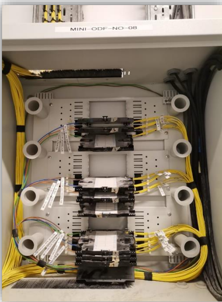
Mini ODF as per DU and Etisalat Standards
