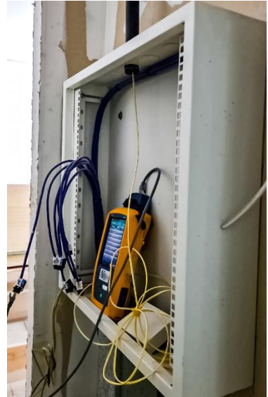
Fluke Testing
