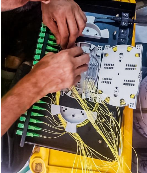
Arrangement of Patch Panel
